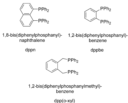
Scheme 2. Nomenclature of the bidentate phosphanes used within this contribution.
