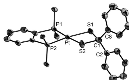
Figure 1. Molecular structure of 6b at 50% probability level. Hydrogen atoms and solvent molecules have been omitted for clarity. The phenyl groups of the dppbe ligand are represented by their ipso -carbon atoms. Selected bond lengths [Å] and angles [°]: Pt–P1 2.257(2), Pt–P2 2.2323(19), Pt–S1 2.324(2), Pt–S2 2.318(2), S1–C1 1.872(9), S2–C1 1.865(8), P1–Pt–P2 87.12(8), S1–Pt–S2 75.86(8), P1–Pt–S1 102.56(8), P2–Pt–S2 94.57(8), S1–C1–S2 99.6(4).
