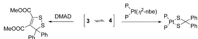
Scheme 6. Comparison of the trapping reactions of diphenylthiosulfine ( 3 ) and diphenyldithiirane ( 4 ) with DMAD and a (bisphosphane) \text{Pt}^0 complex fragment, respectively.
