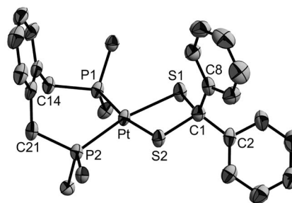
Figure 2. Molecular structure of 6c at 50% probability level. Hydrogen atoms and solvent molecules have been omitted for clarity. The phenyl groups of the dpp(o-xyl) ligand are represented by their ipso -carbon atoms. Selected bond lengths [Å] and angles [°]: Pt–P1 2.2624(12), Pt–P2 2.2613(13), Pt–S1 2.3173(13), Pt–S2 2.3149(12), C1–S1 1.856(5), C1–S2 1.856(5), P1–Pt–P2 95.42(5), S1–Pt–S2 75.99(4), P1–Pt–S1 95.09(5), P2–Pt–S2 93.82(5), S1–C1–S2 100.4(2).
