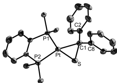
Figure 3. Molecular structure of 7b at 50% probability level. Hydrogen atoms and solvent molecules have been omitted for clarity. The phenyl groups of the dppbe ligand are represented by their ipso -carbon atoms. Selected bond lengths [Å] and angles [°]: Pt–P1 2.2492(18), Pt–P2 2.260(2), Pt–S 2.295(2), Pt–C1 2.156(7), C1–S 1.815(11), P1–Pt–P2 87.34(7), S–Pt–C1 48.0(3), P1–Pt–C1 113.2(3), P2–Pt–S 111.36(7), C2–C1–C8 116.4(7).
