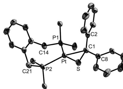
Figure 4. Molecular structure of 7c at 50% probability level. Hydrogen atoms and solvent molecules have been omitted for clarity. The phenyl groups of the dpp(o-xyl) ligand are represented by their ipso -carbon atoms. Selected bond lengths [Å] and angles [°]: Pt–P1 2.2475(13), Pt–P2 2.2733(11), Pt–S 2.2990(14), Pt–C1 2.157(5), C1–S 1.787(5), P1–Pt–P2 102.58(5), S–Pt–C1 47.14(14), P1–Pt–C1 104.07(14), P2–Pt–S 106.21(5), C2–C1–C8 115.4(4).
