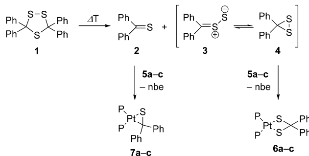
Scheme 5. Postulated mechanism of the formation of dithiolato complexes 6 and \eta^2 -thioetone complexes 7 in the reaction of 1 with 5a–c [a: \text{P} = 1/2 dppn; b: \text{P} = 1/2 dppbe; c: \text{P} = 1/2 dpp(o-xy)].
