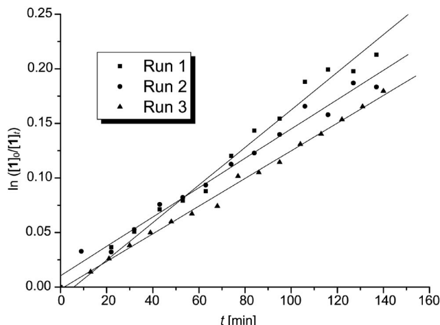
Figure 5. Plot of the natural logarithm of the relative concentration of 1 vs. the time followed by a linear regression of each data set in order to calculate the rate constants based on the concentration of 1 .
